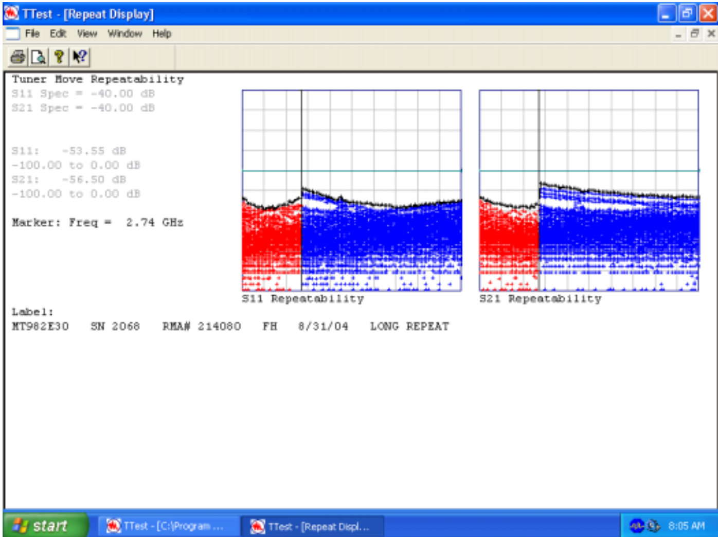
Figure 1. Tuner Repeatability as displayed by the Maury MT993 SNP Software
