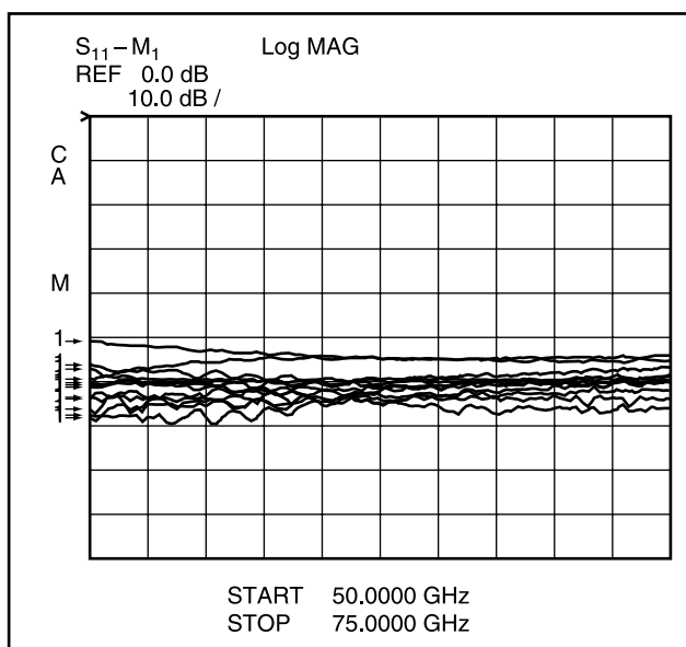
Figure 15. Repeatability of UG385/U Flanges
