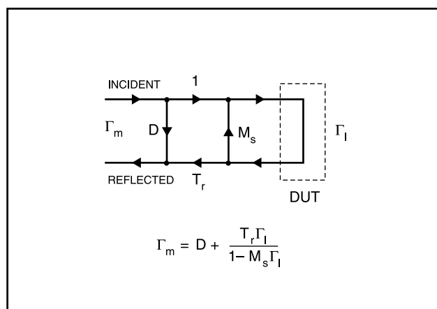
Figure 8. Error Model Modification for One-Port Measurements
