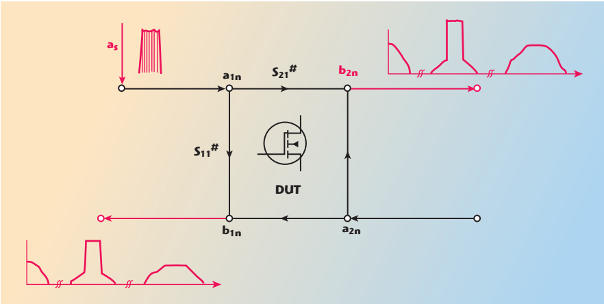
▲ Fig. 11 Signal flow of the original injected signal, reflected signal and amplified signal.
