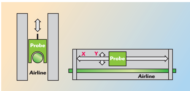
▲ Fig. 7 Cross section and side view of the tuner, slab line and probe.
