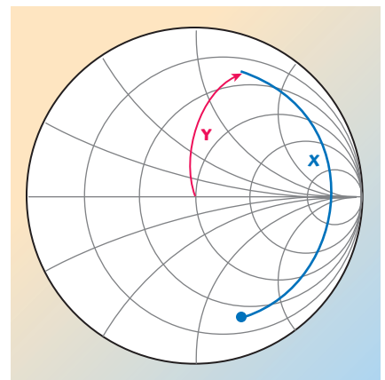
▲ Fig. 8 Impedance change by varying the horizontal (X) and vertical (Y) probe position.
