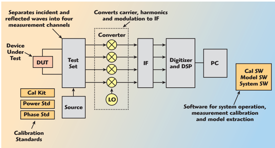
▲ Fig. 5 Functional block diagram of the LSNA.
