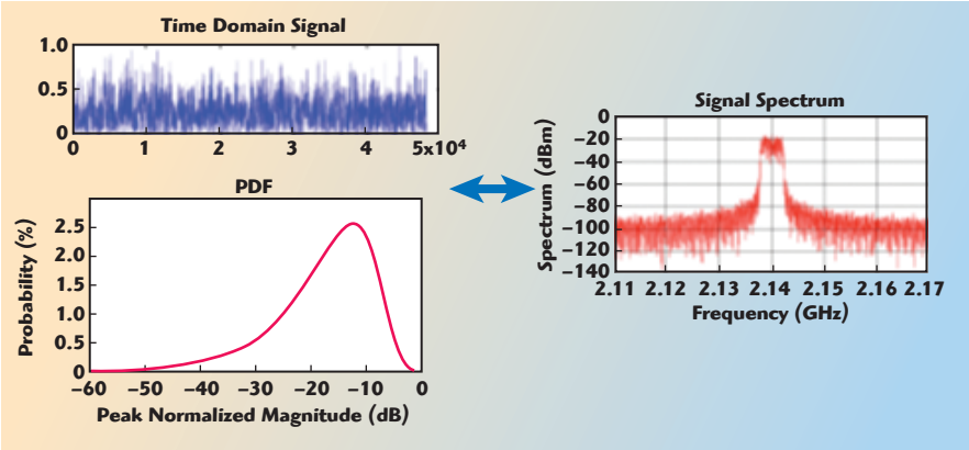
▲ Fig. 10 Realistic wideband signal.
