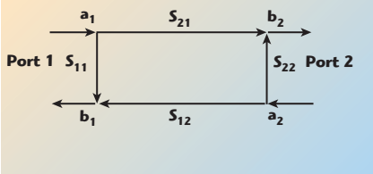
▲ Fig. 1 Generalized two-port network.
