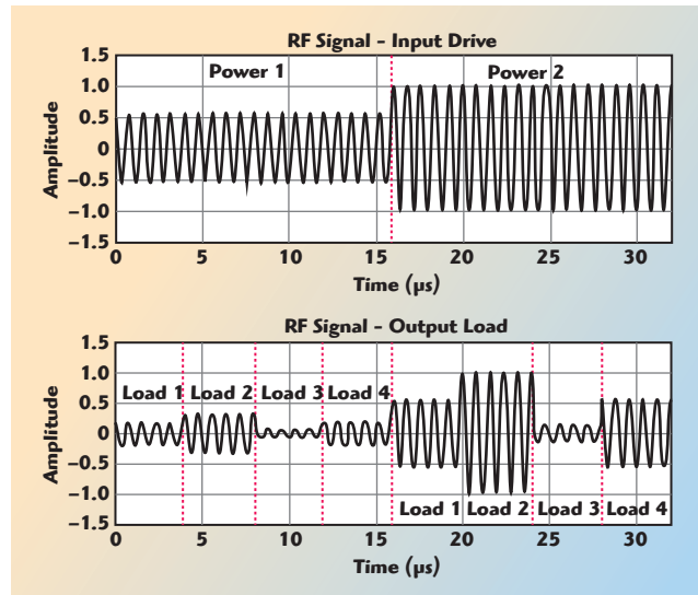
▲ Fig. 13 Time slotting of a CW signal for fast load-pull measurements.
