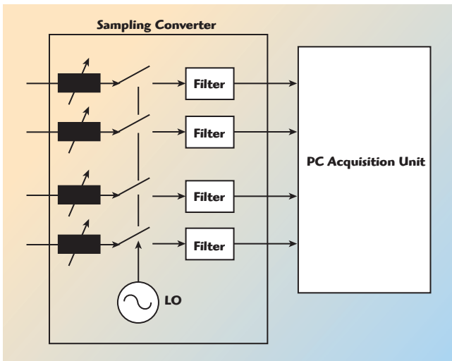
▲ Fig. 6 LSNA sampling converter.
