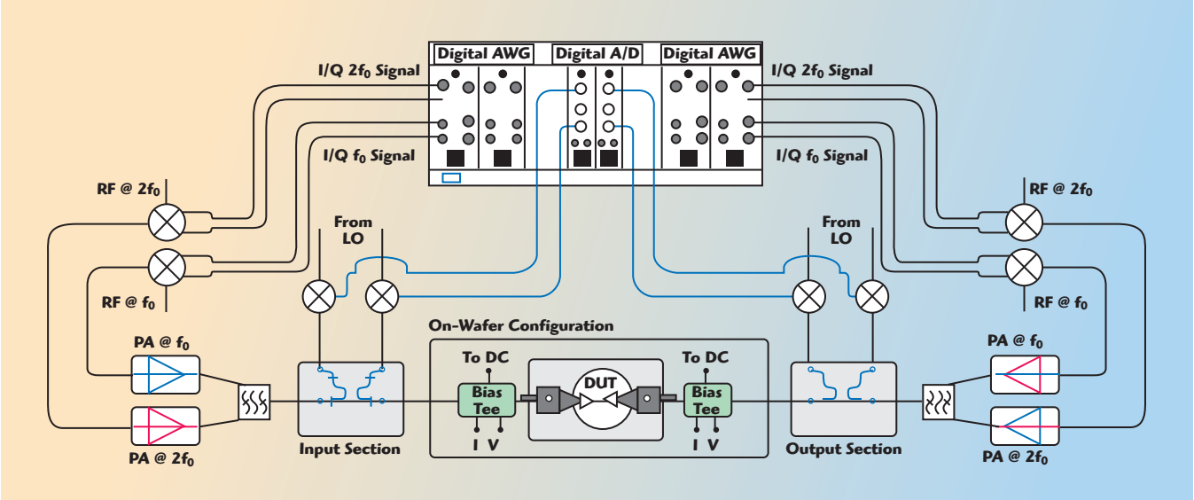
▲ Fig. 9 Functional block diagram of the MT2000.
