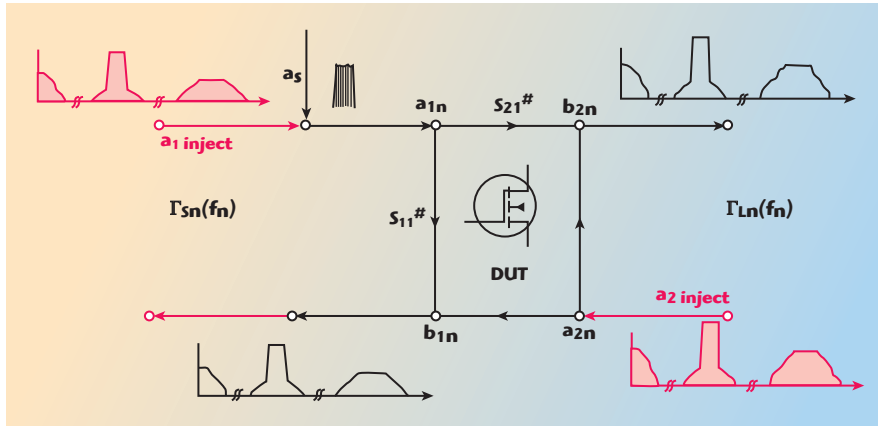
▲ Fig. 12 Signal flow of the original injected signal, reflected signal and amplified signal (black) and the generated signals for active tuning (red).
