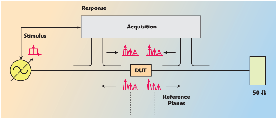
▲ Fig. 4 Signal flow of LSNA with exemplary 50 ohm termination.
