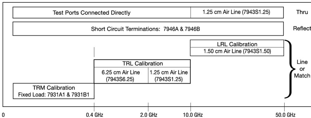
Figure 2. TRM/TRL/LRL Calibration
