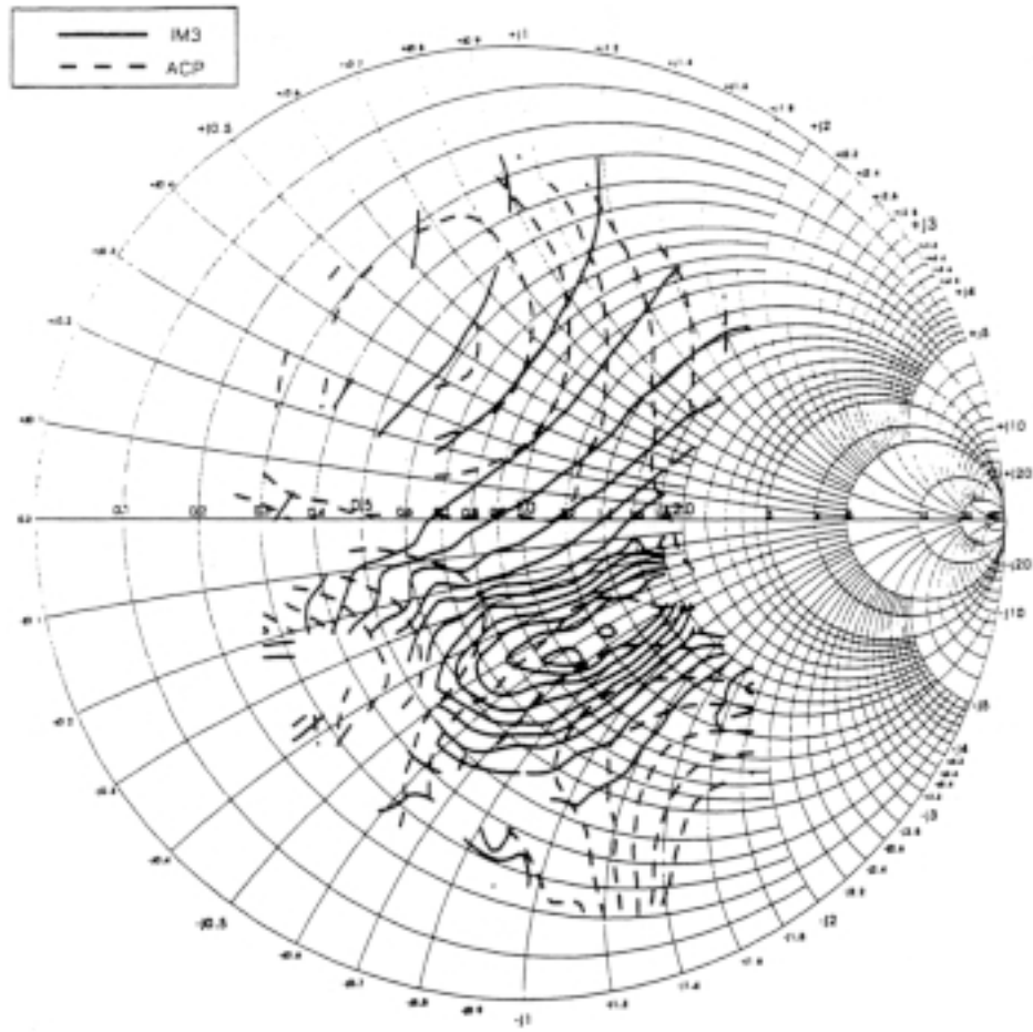
Figure 2: Third-order IM and ACP contours for the GaAs MESFET.
