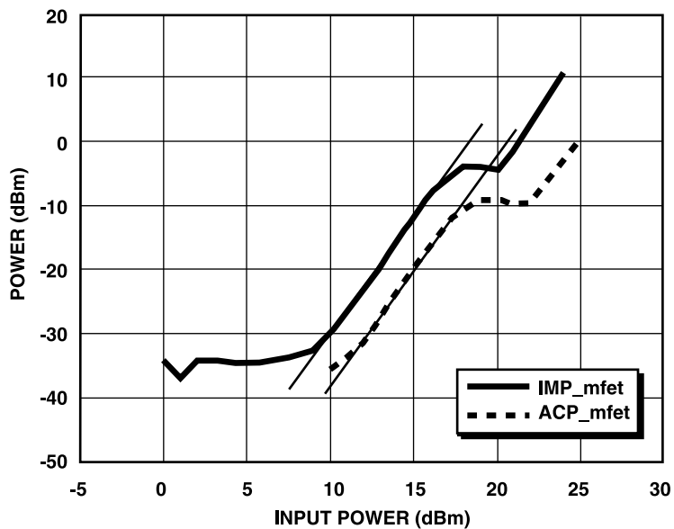
Figure 5: Comparison of third-order IM power and adjacent-channel power for GaAs HEMT.
