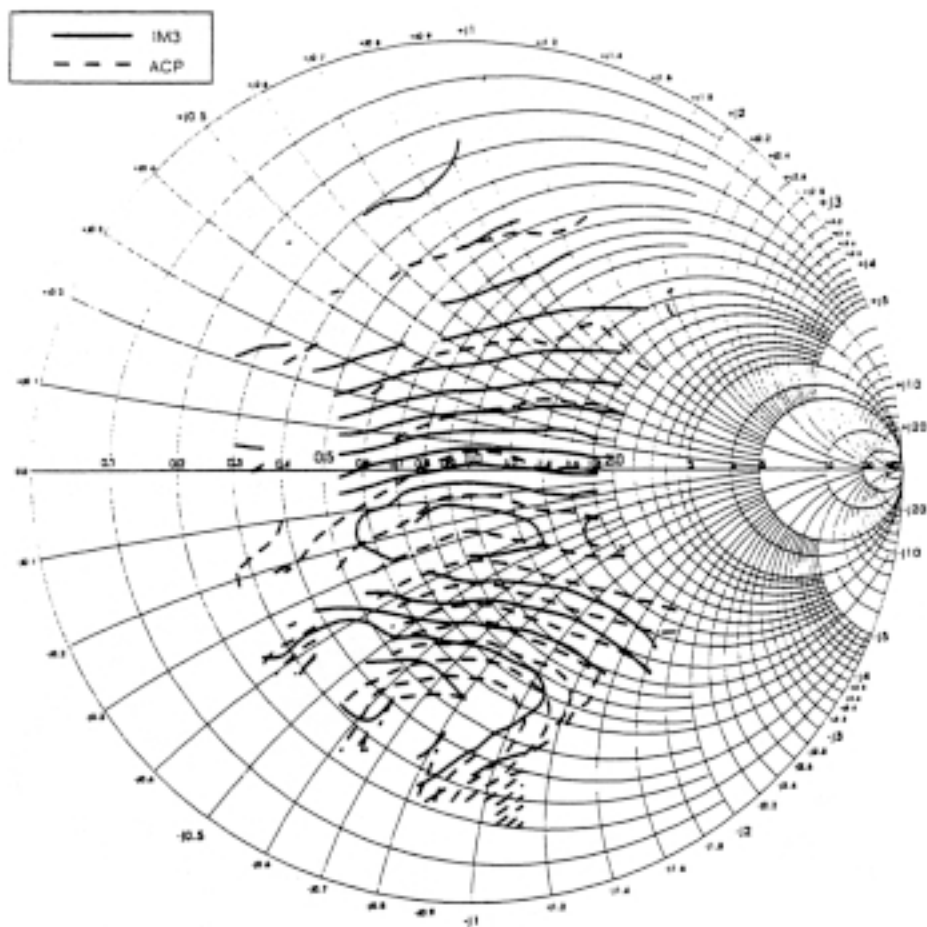
Figure 4: Third-order IM and ACPR contours for the GaAs HEMT.
