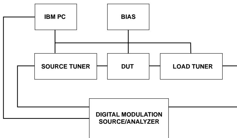
Figure 1: Diagram of the automated large-signal load-pull system.
