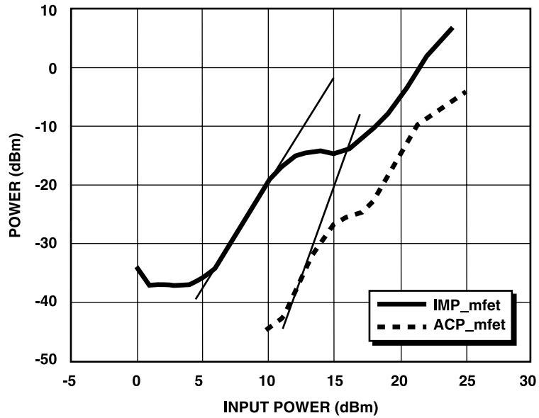
Figure 3: Comparison of third-order IM power and adjacent-channel power for GaAs MESFET.
