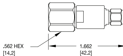
Model 8025D1 (TNC male to 3.5mm male adapter)
