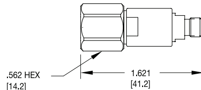
Model 8025B1 (TNC male to 3.5mm female adapter)
