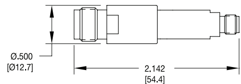
Model 8025A1 (TNC female to 3.5mm female adapter)
