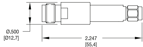
Model 8025C1 (TNC female to 3.5mm male adapter)
